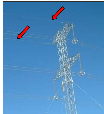
The 66 kV Trekkopje Bypass line (right, with wooden five-pole structures) runs parallel to the larger 220 kV line (left); it is possible that the three flamingos collided with the less visible earth/optic fibre ground wires (red circle above and red arrows below) on the latter structure (photos Ann Scott)
